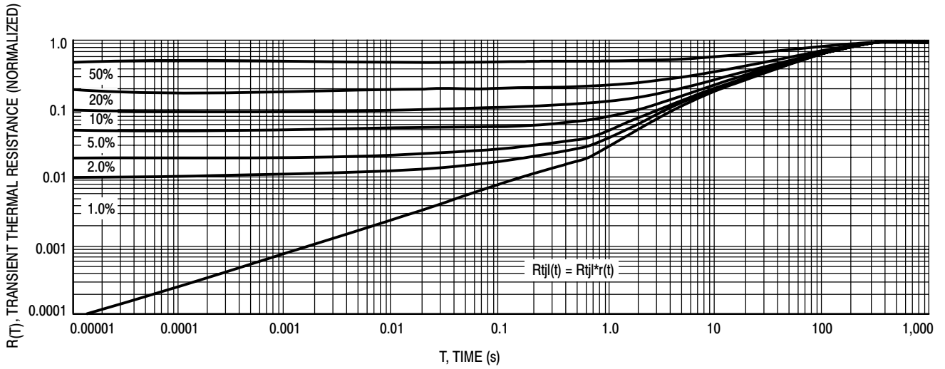
Figure 10. Thermal Response Junction to Ambient (Per Leg)
